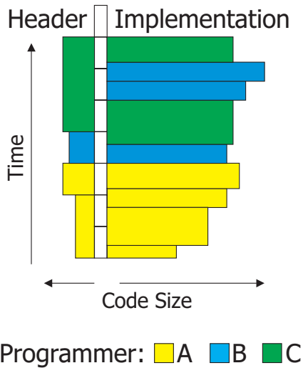
Fig. 5.6. Revision tower: evolution of a C file and its header file
