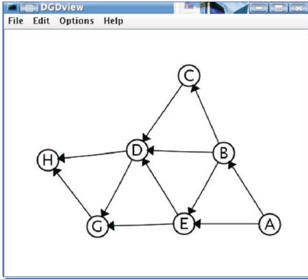
Fig. 2.9. Force-directed layout
