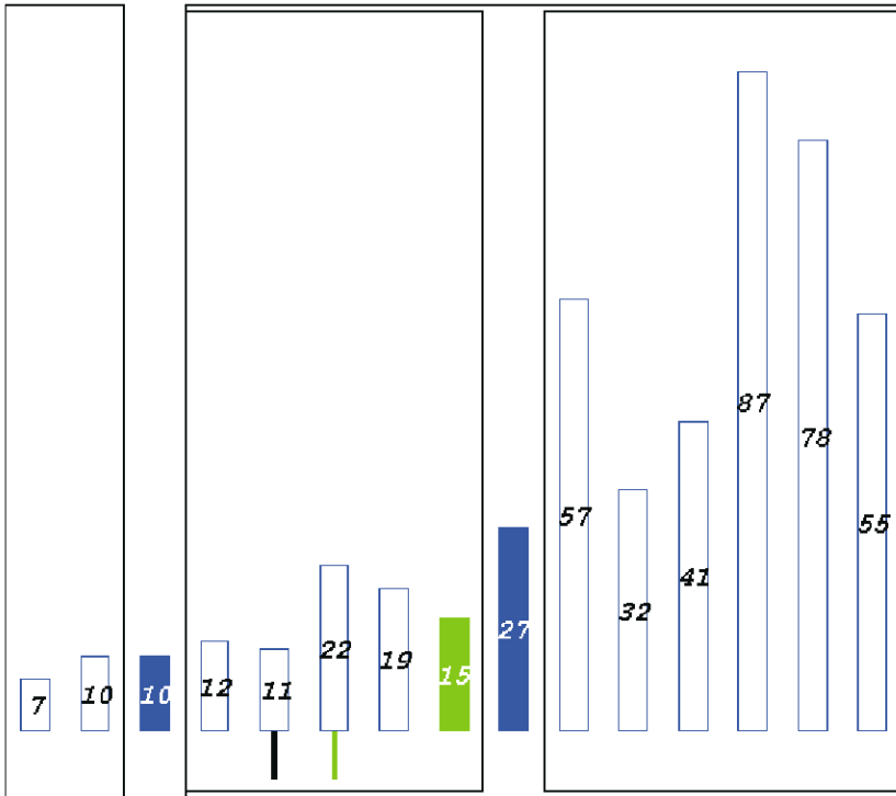
Fig. 4.14. Quicksort algorithm
