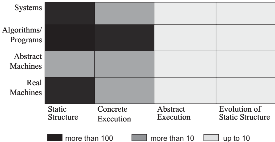
Fig. 1.8. Literature survey
