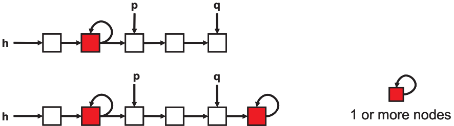
Fig. 4.19. Abstract execution of q := q \rightarrow next
