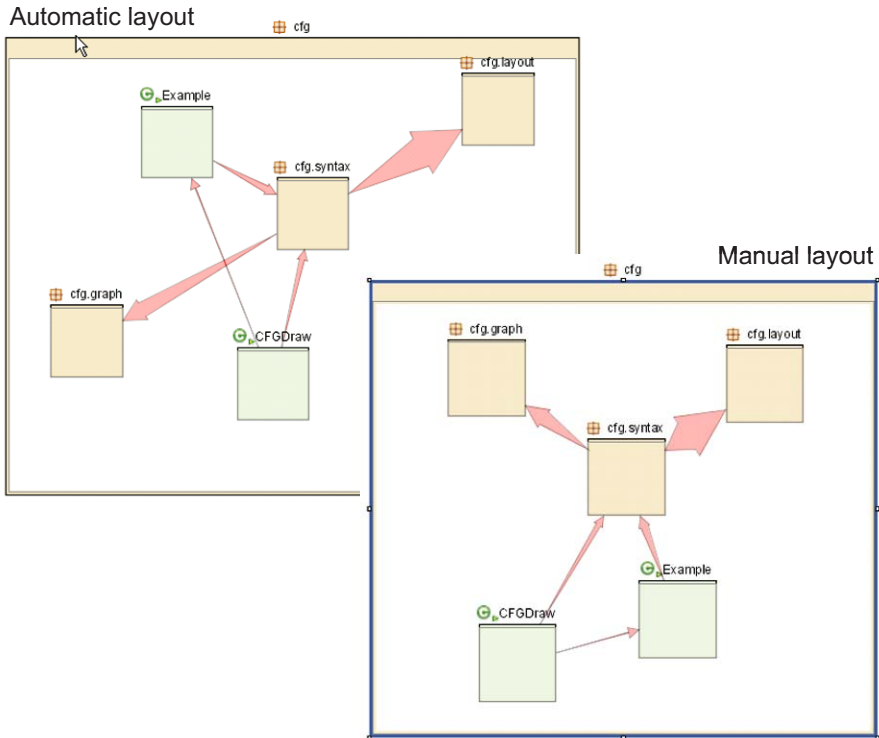
Fig. 3.36. Creole: package dependencies via method calls and field access
