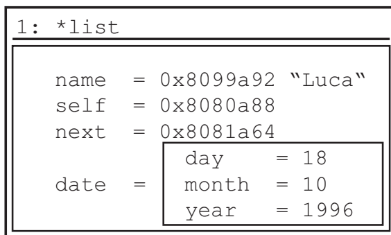
Fig. 4.25. Nested boxes as drawn by DDD
