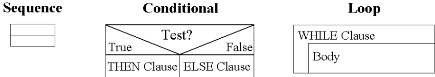
Fig. 3.14. Basic Nassi-Shneiderman diagrams
