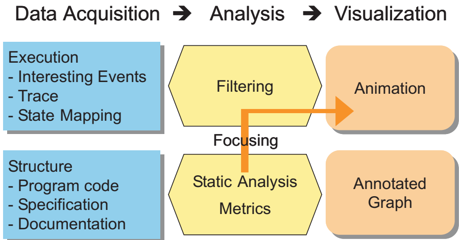
Fig. 4.18. Using program analysis to focus algorithm animations
