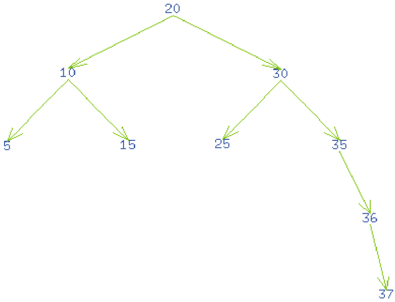
Fig. 4.9. Binary tree
