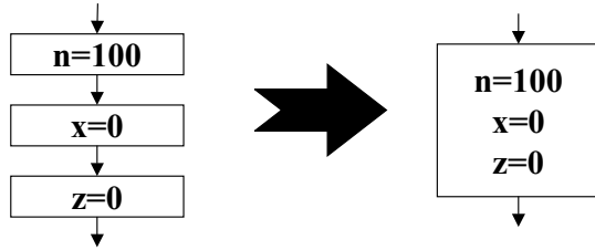
Fig. 3.8. Basic block
