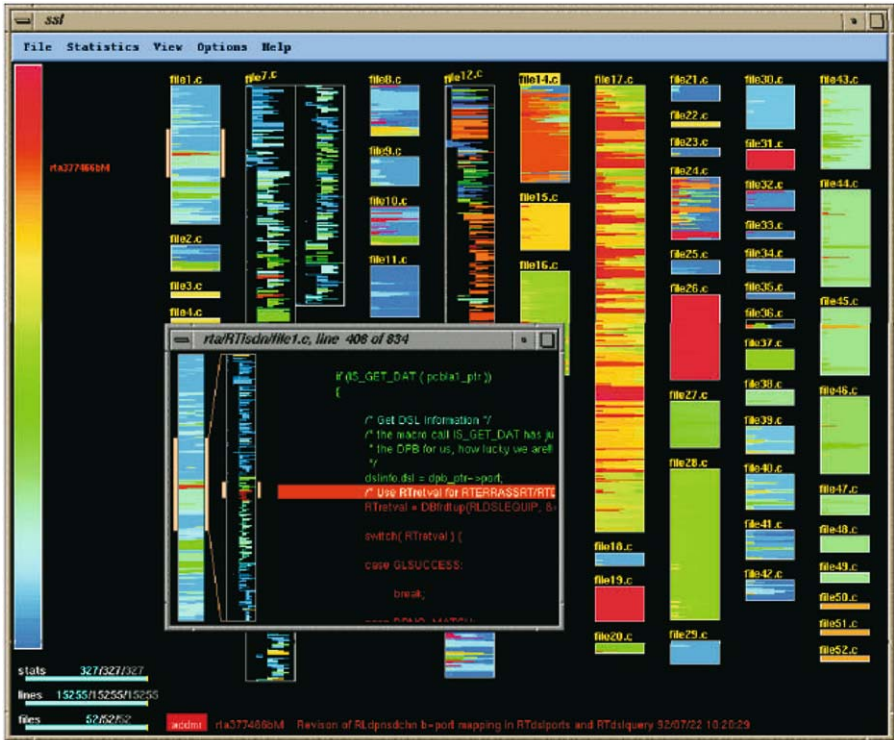
Fig. 1.6. Visualizing the age of program code changes (©1996 IEEE)
