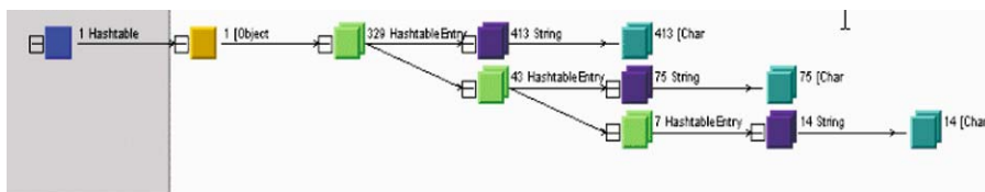
Fig. 4.31. Reference pattern extracted for a hash table
