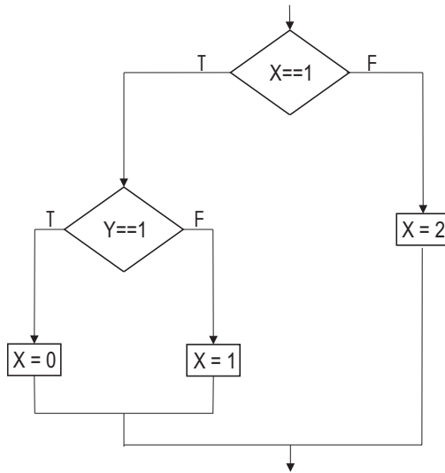
Fig. 3.41. Control-flow graph for Exercise 2
