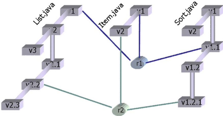
Fig. 5.9. 3D representation of revision tree and releases
